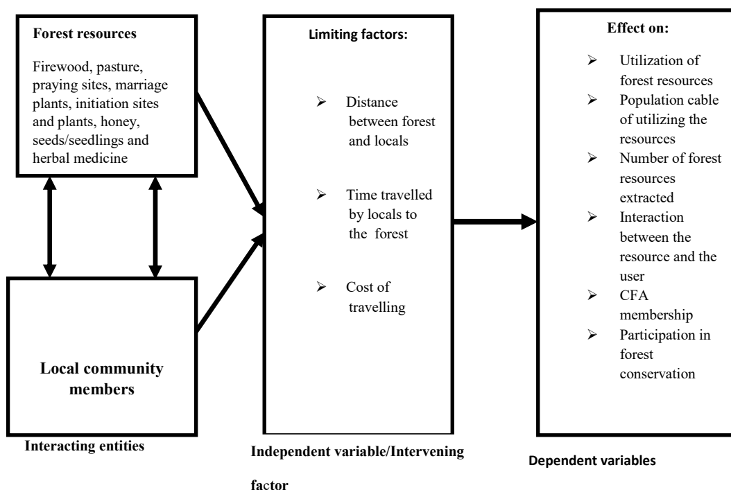
Figure 1: Conceptual frawormework
